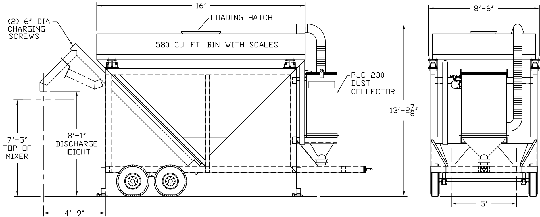
ARROWHEAD MOBILE SILO
